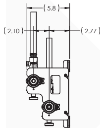
Shown with optional inlet plugs, fittings, outlet plugs; valves not included in EV9662-00
